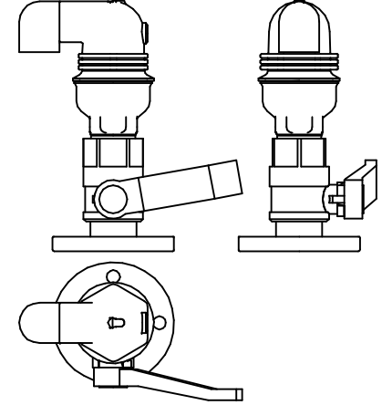
D-040 DN50 WITH TAP&FLANGE
