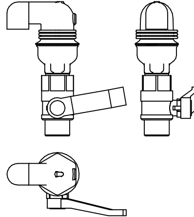
D-040 DN50 WITH TAP
